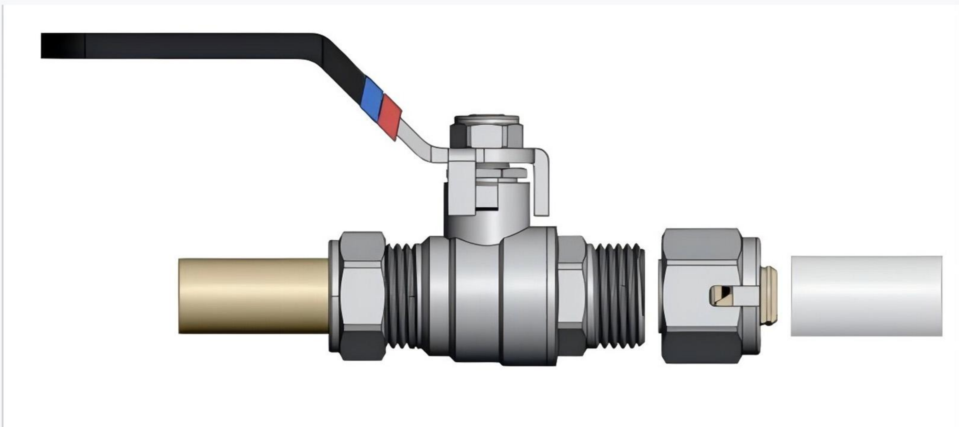
Compression connection on a lever valve with MLCP pipe - exploded view
