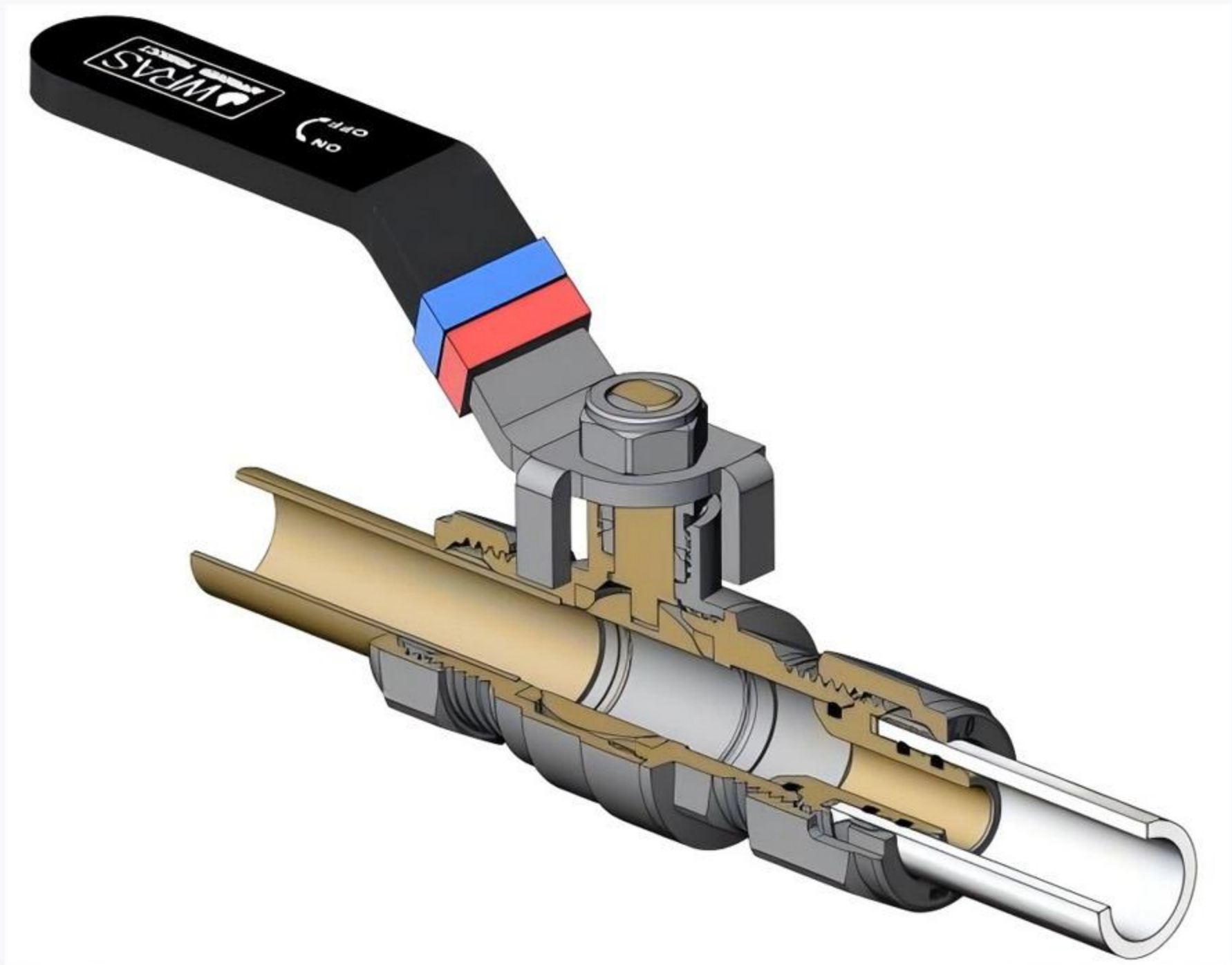
Cutaway view of the compression joint
