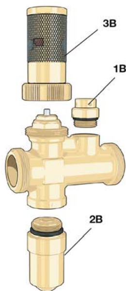
Antifreeze valve with air sensor
